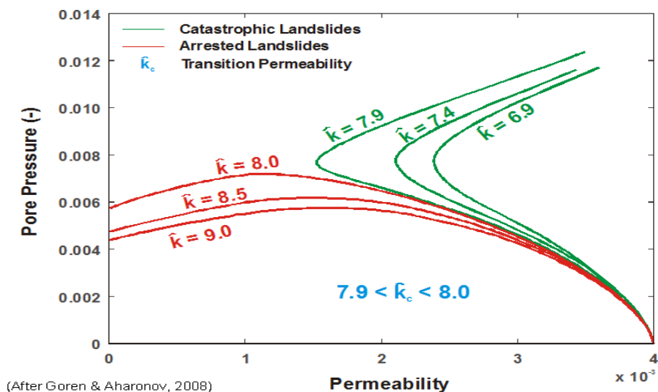
Figure 2 Effects of permeability ratios on pore pressure dissipation and shear movements (Goren and Aharonov 2008).
