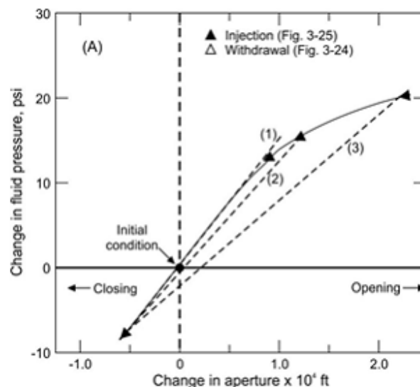
Figure 3 Changes in fracture aperture due to changes in borehole packer injection pressures.
