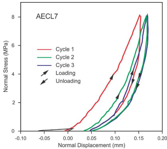
Figure 5 Measured fracture closure as a function of normal stress showing decrease in hysteresis and permanent deformation with repeated loading cycles (After Gale et al. 2001).
