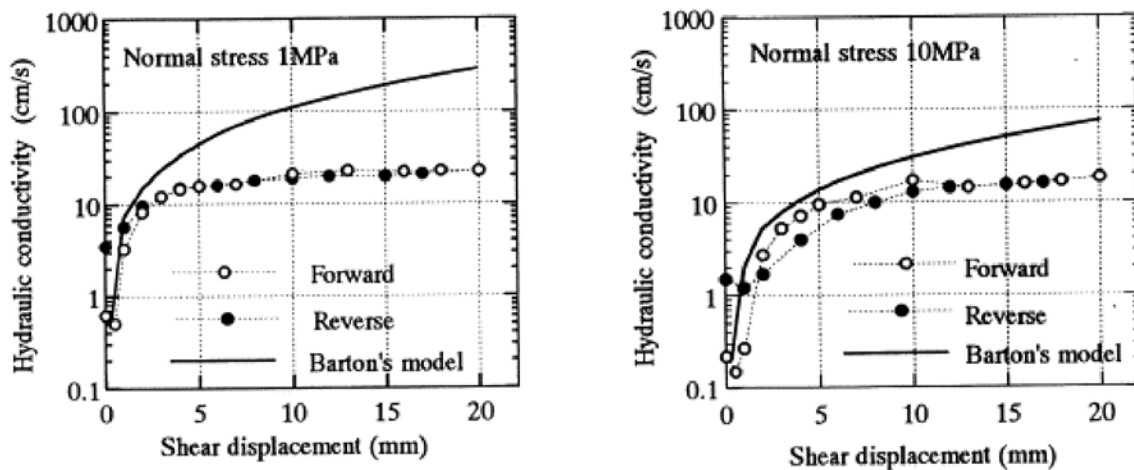
Figure 6 Hydraulic conductivity of a granitic joint as a function of shear displacement under a normal stress of (a) 1 MPa and (b) 10MPa, Esaki et al. (1999).
